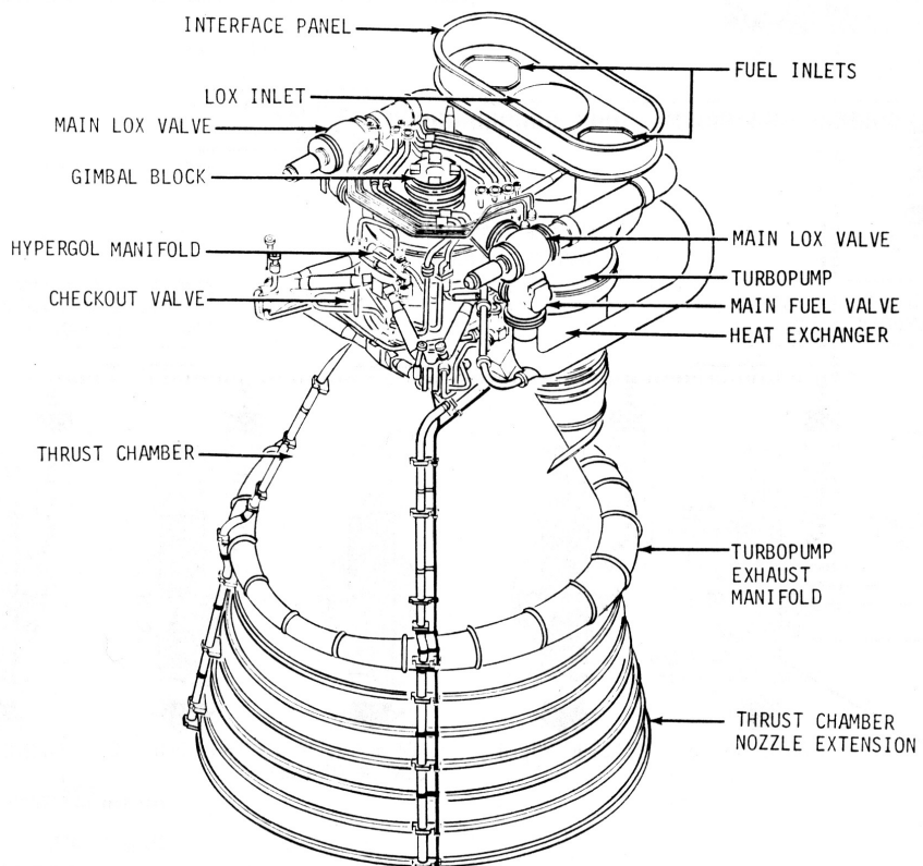
Figure 41: F-1 operation schematic [155].
